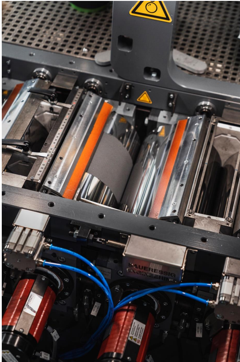
A fine coating film forms on the faster-rotating roller. © Fraunhofer IWS Dresden
