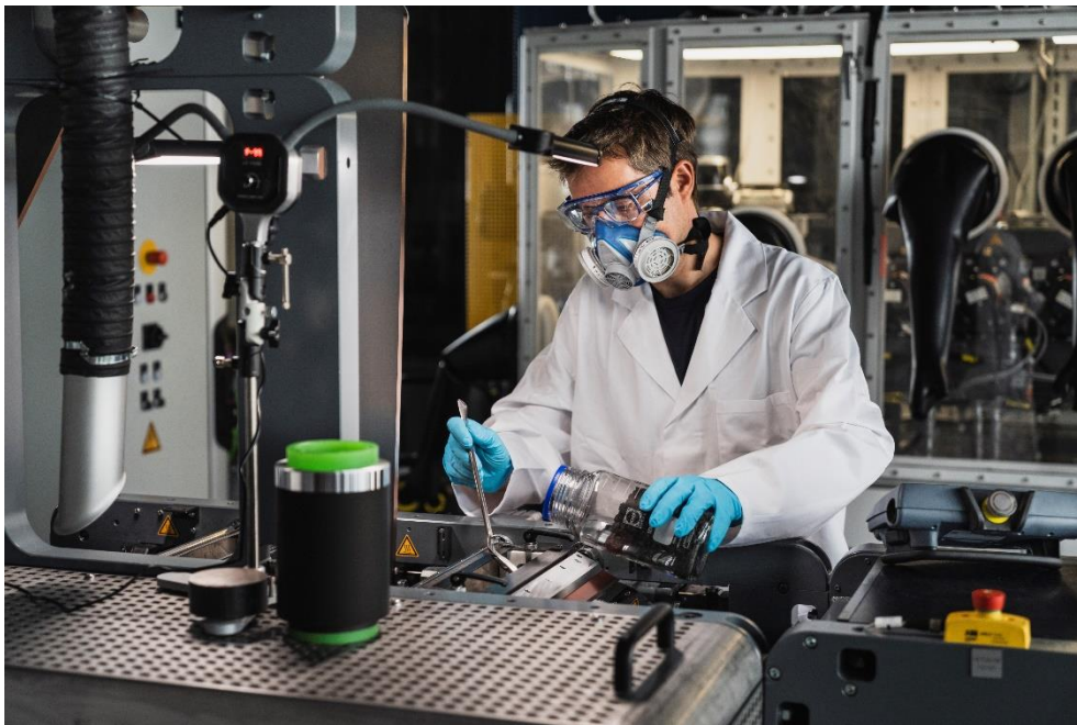
The dry coating powder is fed into the calender gap in the DRYtraec® machine. © Fraunhofer IWS Dresden
